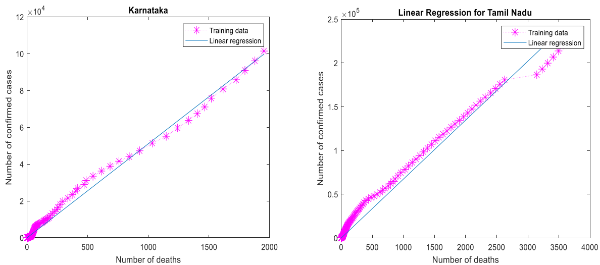
Figure 3: Linear Regression for Karnataka and Tamil Nadu.
