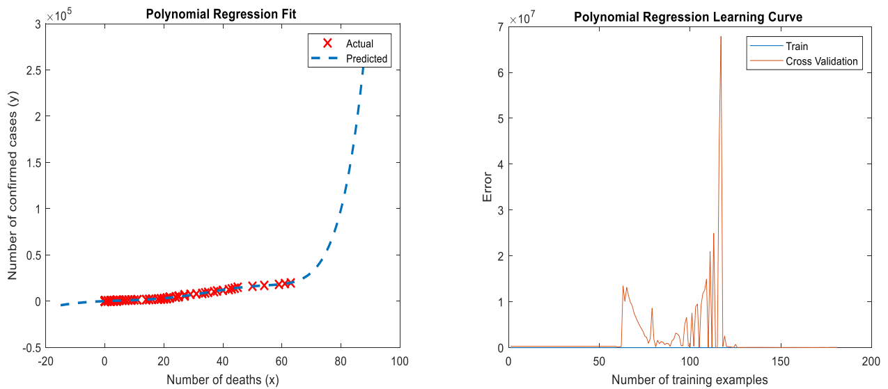
Figure 8: Polynomial Regression fit for state of Kerala and Polynomial learning Curve.
